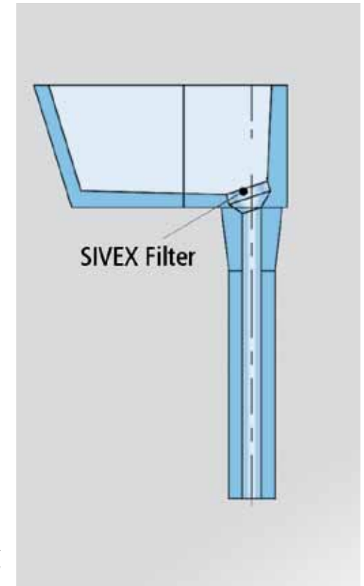
Filter funnel used to pour molten metal into low pressure or bale-out furnaces
