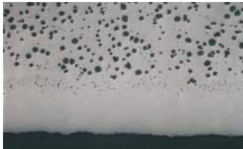
Unlike exothermic alternatives, the steel breaker core has no adverse effects on SG iron structure
