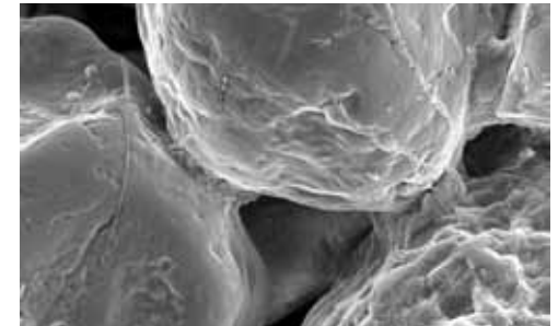
SEM photo of silicate bonded sand
